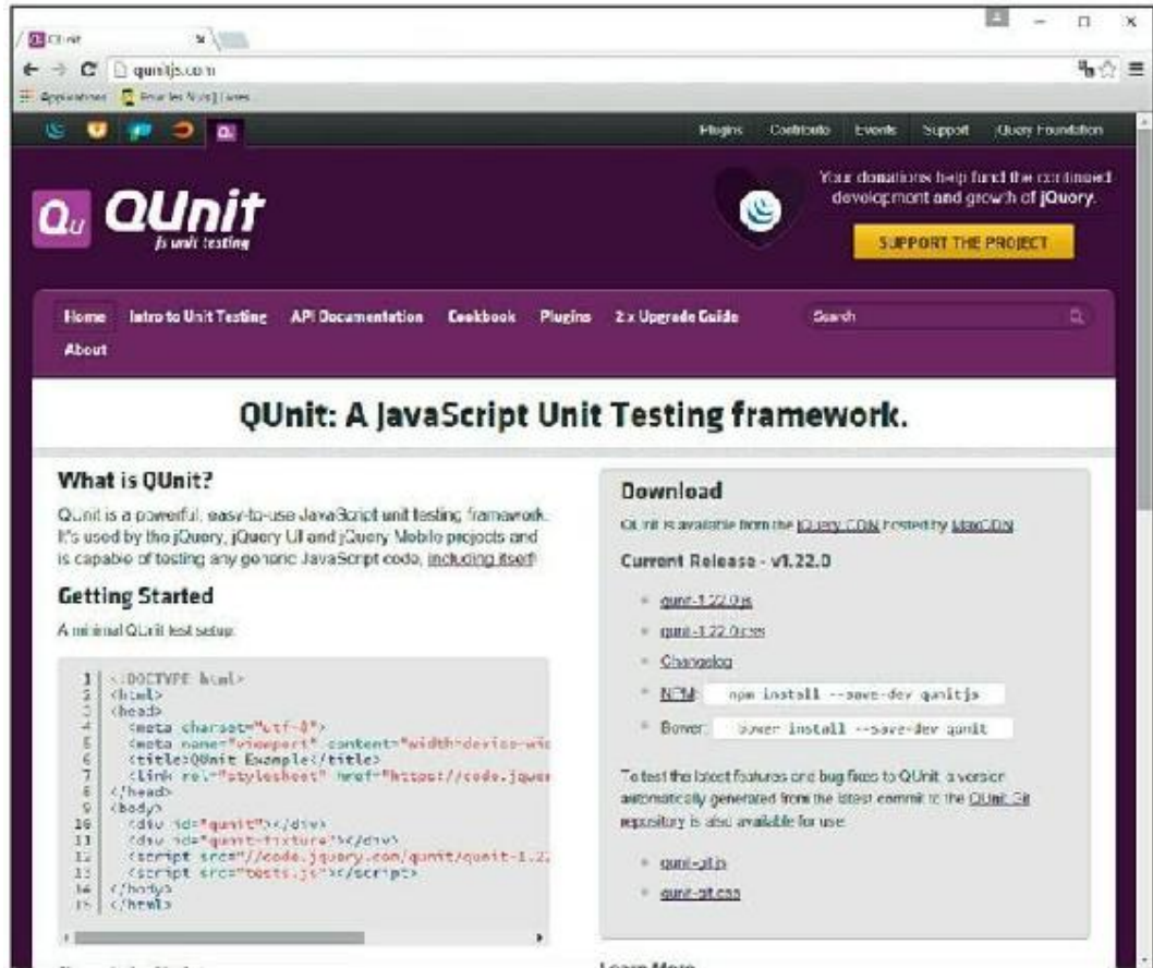
FIGURE 19.6 : http://qunitjs.com .
