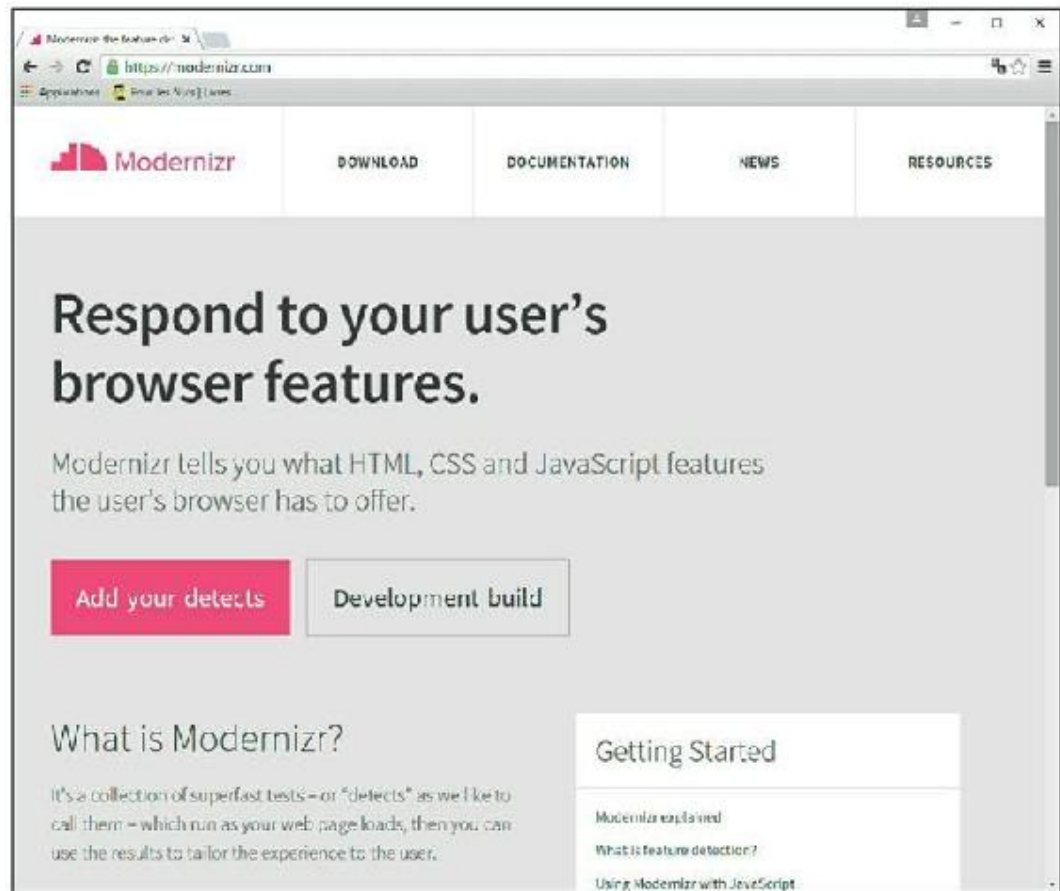
FIGURE 19.8 : http://modernizr.com .
