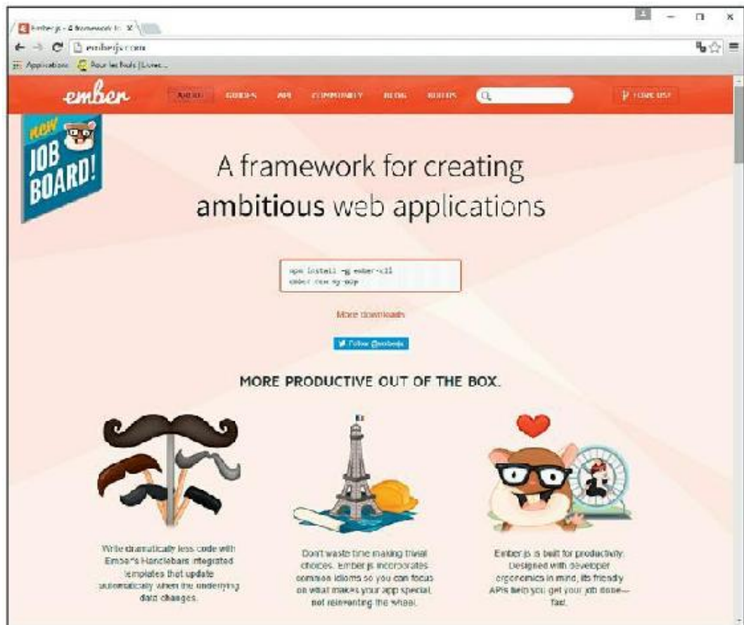
FIGURE 19.3 : http://emberjs.com .
