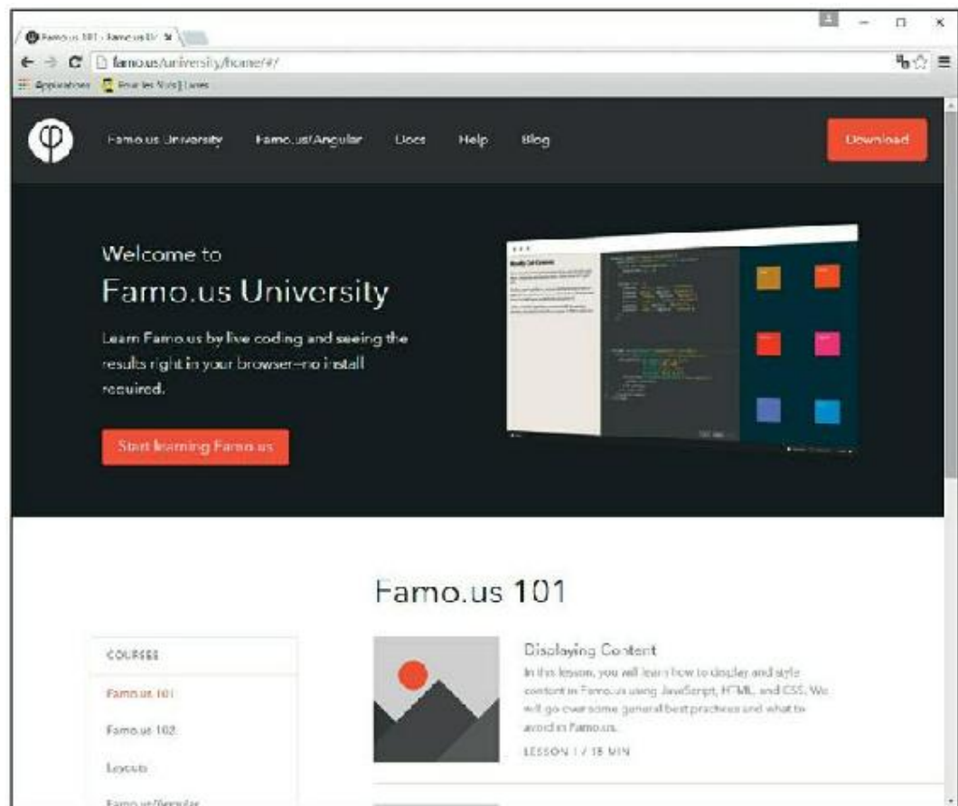
FIGURE 19.4 : http://famo.us .
